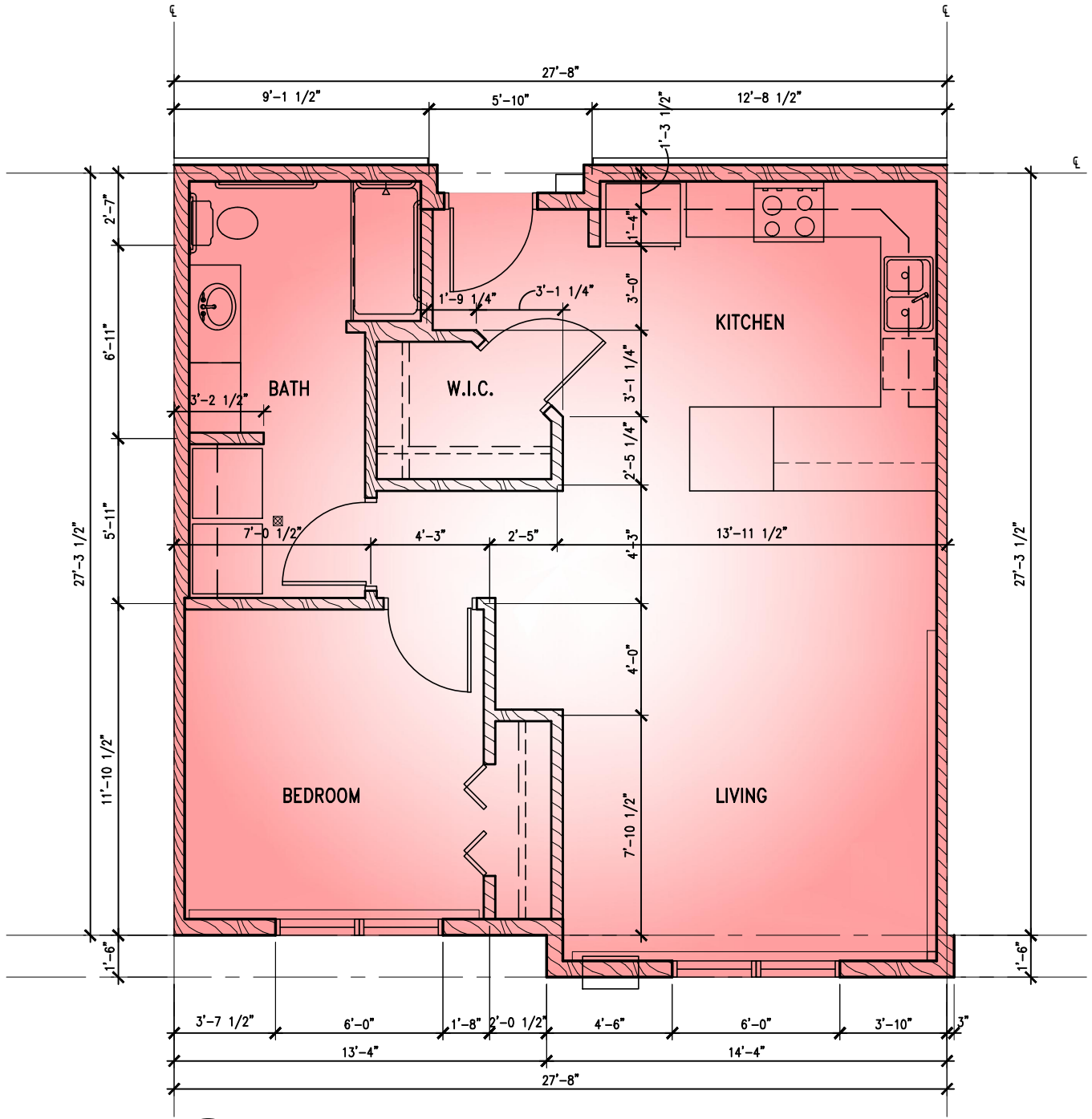
4 UNIT D-1 PLAN A340 1/4" = 1'-0" TYPE B UNIT
