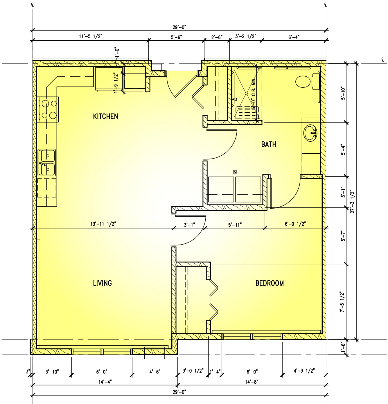
1 UNIT A-1 PLAN A340 1/4" = 1'-0"
