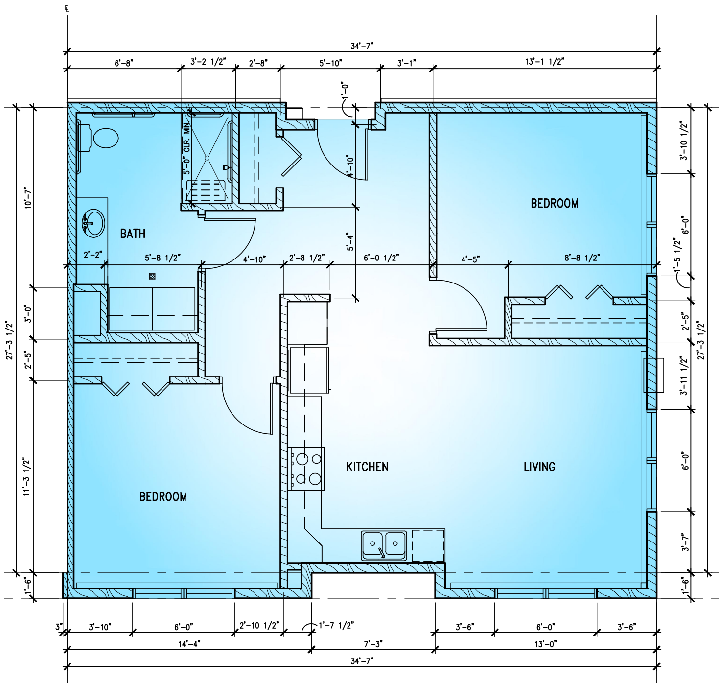
3 UNIT C-2 PLAN A340 1/4" = 1'-0"
