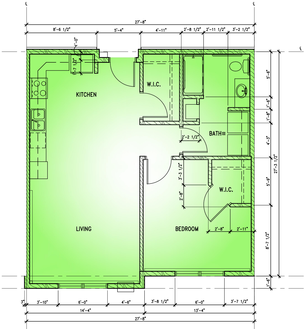
2 UNIT B-1 PLAN A340 1/4" = 1'-0"
